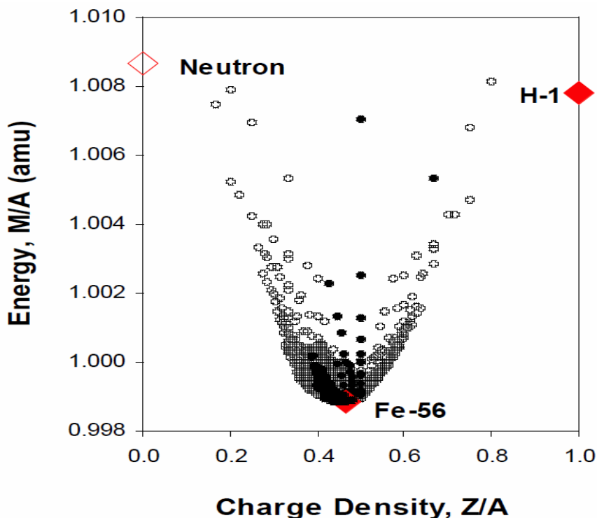
Figure 1a: Two forms of one fundamental particle shown by the red symbols on the left (neutrons) and right (hydrogen atoms, H-1) comprise every atom. The most stable atom, Fe-56, is also the most abundant atom in the Earth, in the Sun and in ordinary meteorites. On Earth H-1 is more stable than the neutron. At high pressure, H-1 atoms collapse into neutrons [17] and can be energized by neutron repulsion to energy levels above the top of the page [12].
