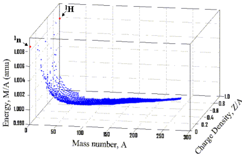
Figure 1b. Combinations of the two forms of one particle that comprise all of the atoms, neutrons ( ^1n ) in the front and hydrogen atoms ( ^1H ) in the back, are sorted above by mass number ( A ) on the horizontal axis and by charge density ( Z/A ) in the third dimension.
