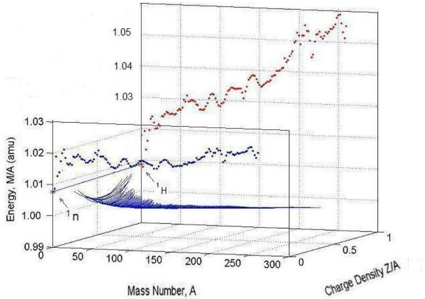
Figure 1c. Parabolas defined by mass data points reveal maximum: Neutron repulsion at Z/A = 0 (o) on the front panel (nuclei made of neutrons only); Proton repulsion at Z/A = 1.0 (o) on a back panel (nuclei made of protons only); Differences from Coulomb repulsion [15]; Neutron-proton attraction at Z/A = 0.5
