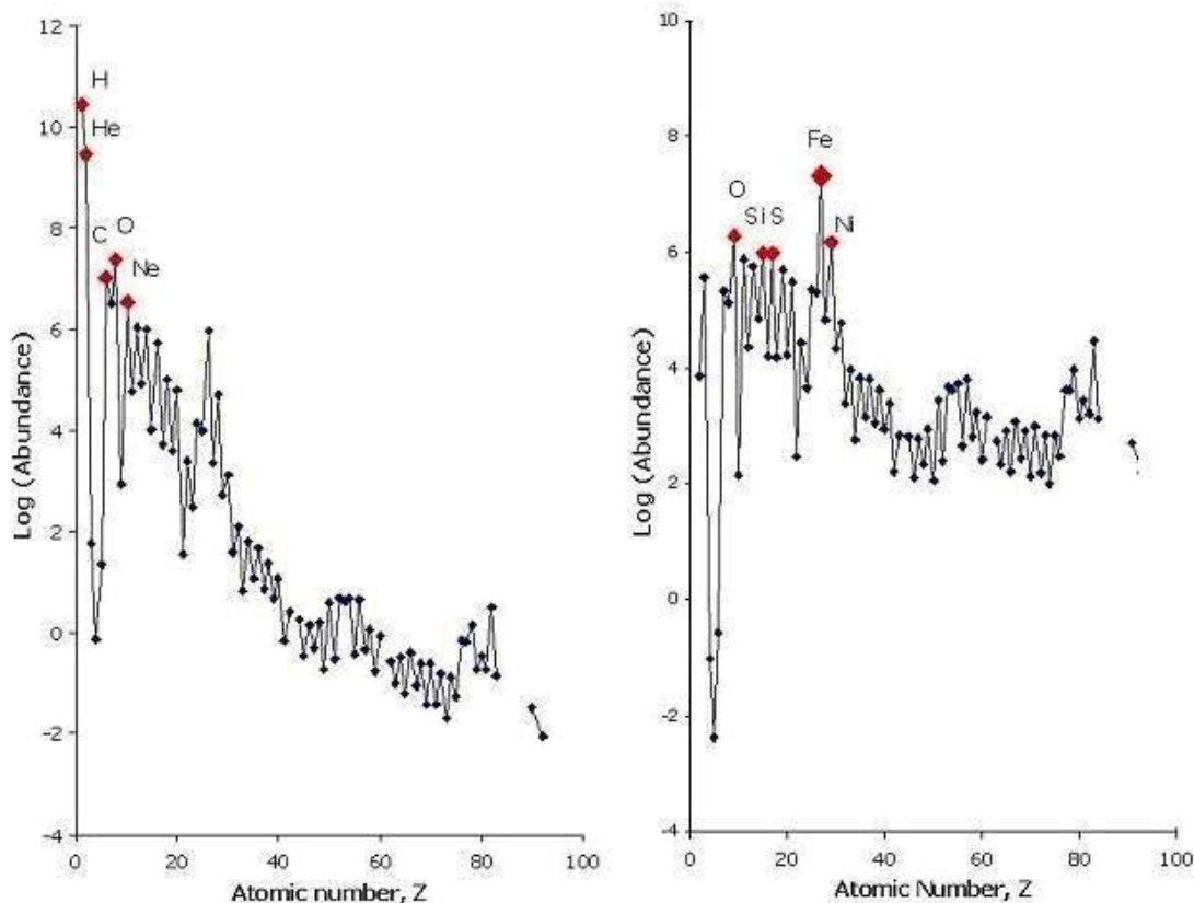
Figure 3b: The severely mass fractionated abundance pattern of elements at the top of the Sun [38] ( left ) becomes remarkably like the abundance pattern of elements on Earth and in ordinary meteorites [39] ( right ) - consisting mostly of Fe, O, Ni, Si and S - after correcting for the severe solar mass fractionation revealed by precise measurements [11] at the Universität Bern, Physikalisches Institut of isotopes implanted in lunar soil #bb18. Correcting for mass fractionation ( Figure 3a, right ) across the 72 s-products that B2FH [27] reported in the solar photosphere in 1957, yields the same five elements - Fe, O, Ni, Si and S - dominant in the interior of the Sun as were revealed by wet chemical analysis as the five most abundant elements in ordinary meteorites forty years earlier, in 1917 [39].
