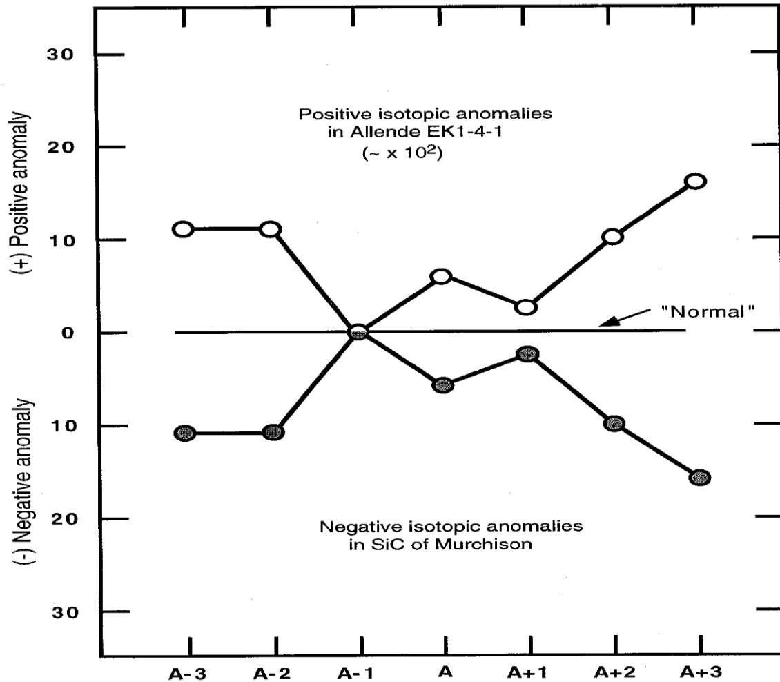
Figure 2d: In 1978 Srinivasan and Anders [28] found a "complementary" component to "strange" xenon, enriched in middle isotopes by the s-process of nucleosynthesis [27], in the Murchison meteorites. By 1993, "strange" and "complementary" isotopic anomalies had been found in the isotopes of xenon (element #54) [18, 28], tellurium (element #52) [21], barium (element #56), neodymium (element #60) and samarium (element #62) [23]. These two anomaly patterns are usually observed in refractory grains of diamond (C) and silicon carbide (SiC) that condensed early in the heterogeneous solar nebula [12, 20, 21].
