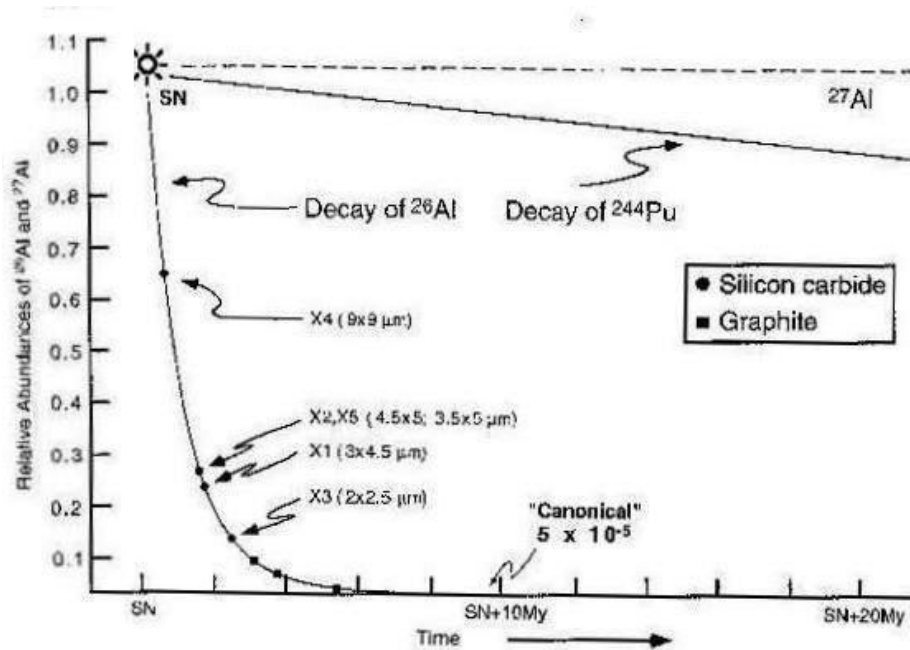
Figure 2f: ^{26}\text{Al}/^{27}\text{Al} age dating of refractory meteorite inclusions of silicon carbide and graphite show that they formed within 1-10 My of the supernova with physical properties like those of "fall-out" particles from nuclear explosions [25]. The grains that formed first grew larger and trapped higher levels of radioactive ^{26}\text{Al} ( t_{1/2} = 740,000 yr or 0.74 my).
