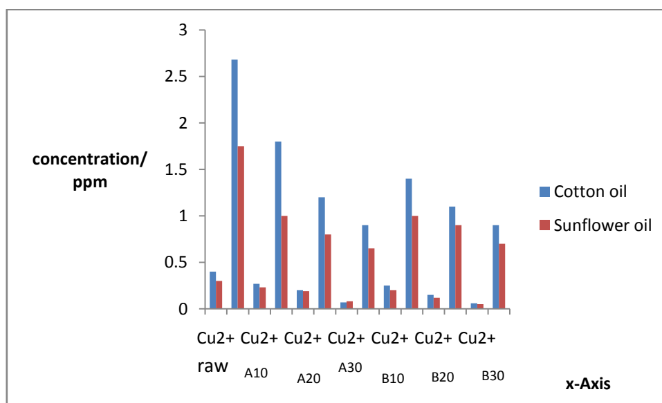
Figure 1: Content of trace metals in bleached oils using Iliri clay activated at 90°C
