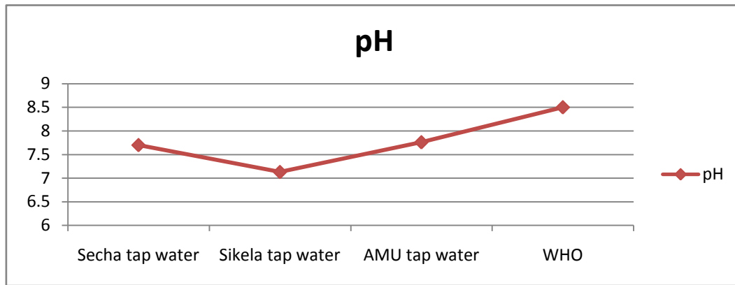
Figure 1: pH values of various water samples
