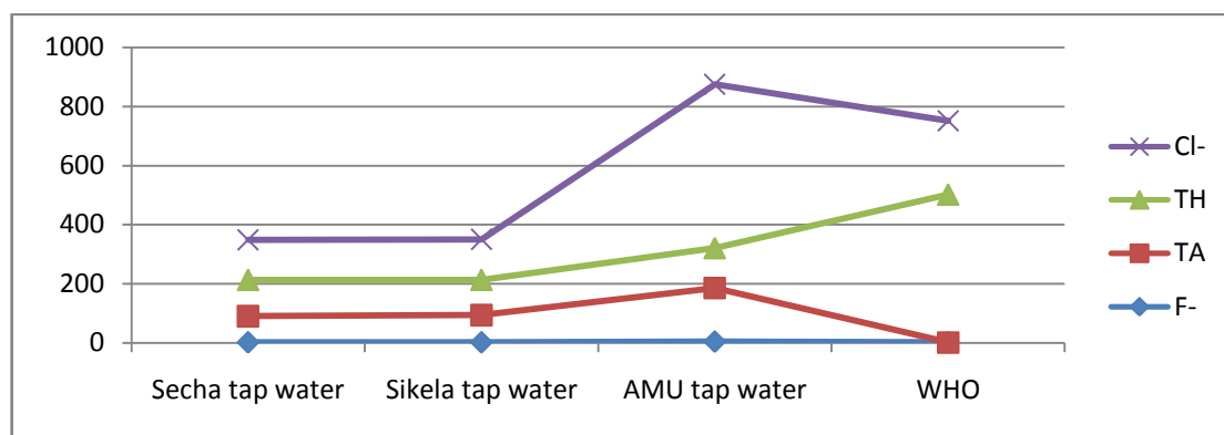
Figure 4: F - , TA, TH and Cl - values of various water samples (all are in mg/L)
