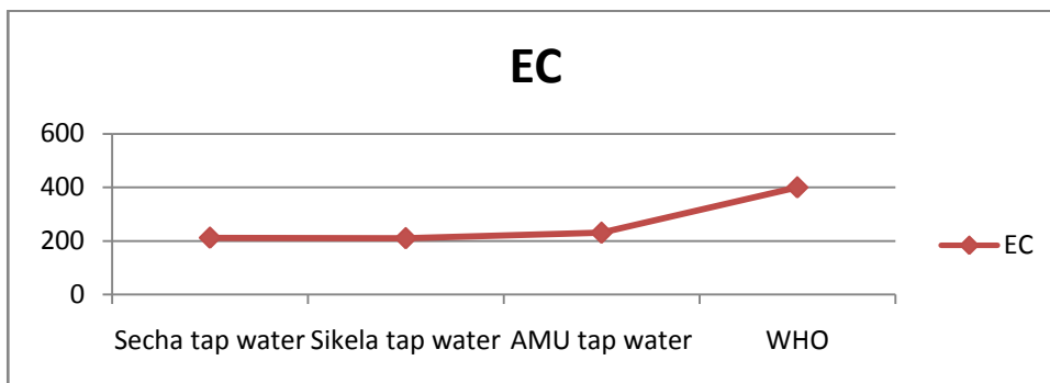
Figure 3: EC values of various water samples in \mu\text{S cm}^{-1}
